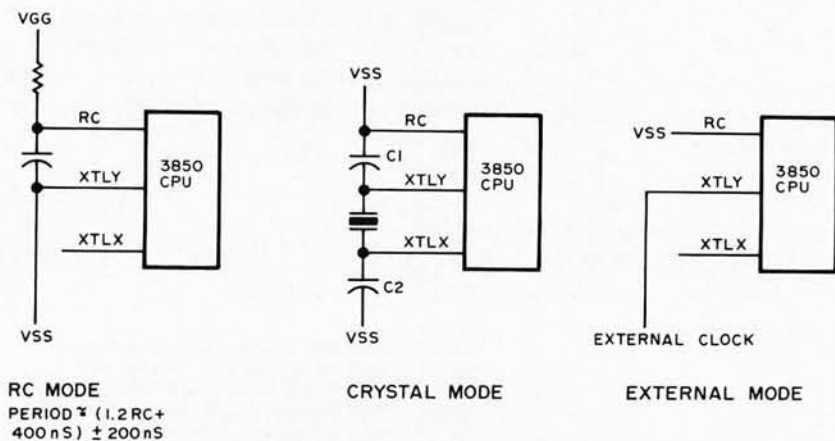
Figure 2: Three modes of clock generation for the F8 system.
